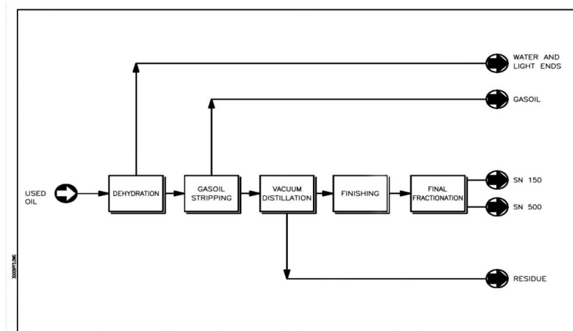
Fig (13) - The STP Process - Source 94
