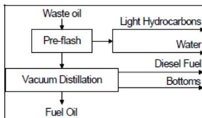
Fig (16) – Trailblazer Process – Source 107
