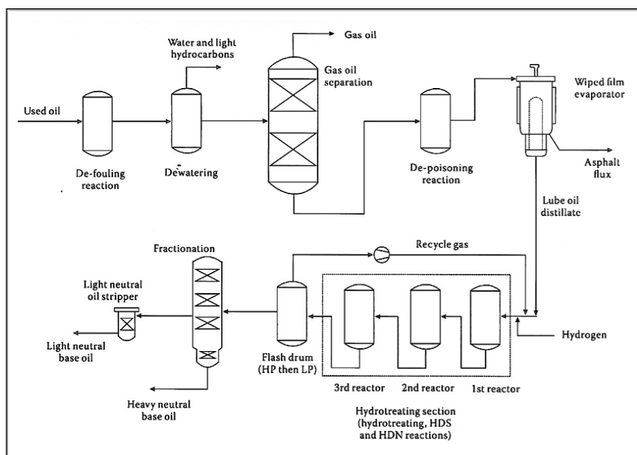
Fig (6) - CEP Mohawk Process - Source 1
