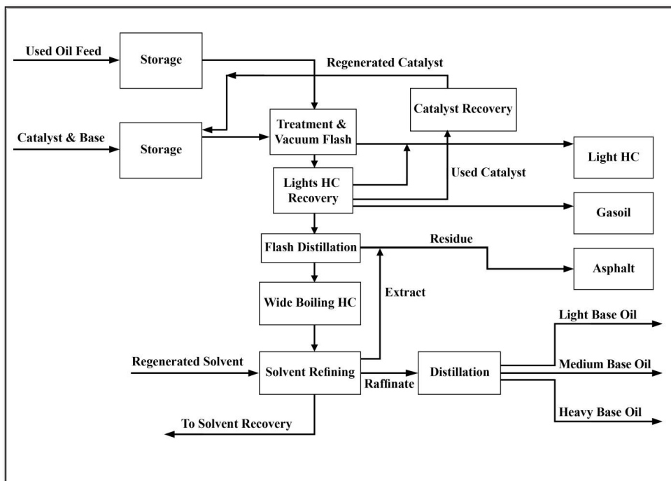
Fig (7) - Avista Process - Source 3
