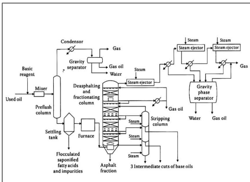
Fig (8) - Original Viscolube Process - Source 1
