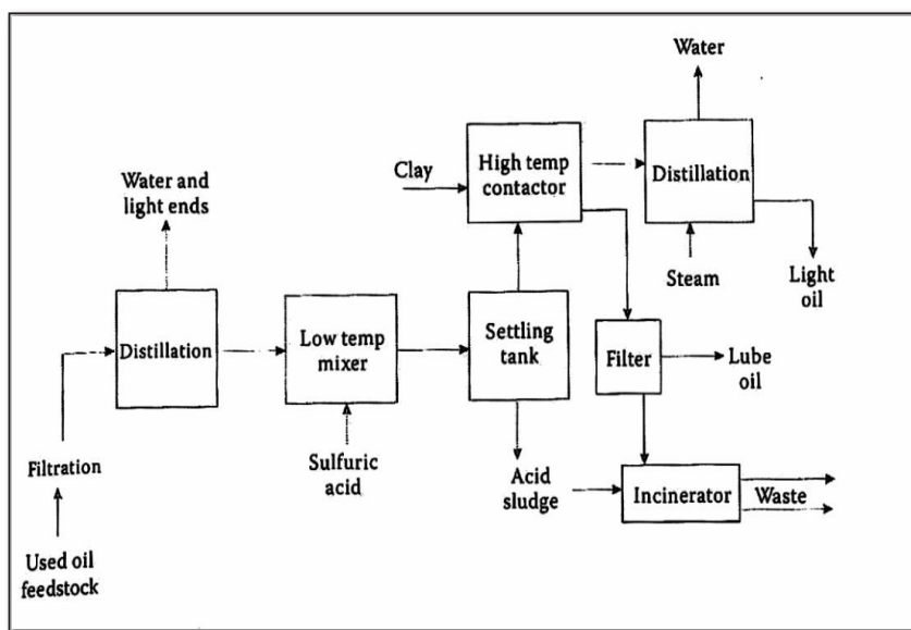
Fig (3) - Acid/Clay Process - Source: 1
