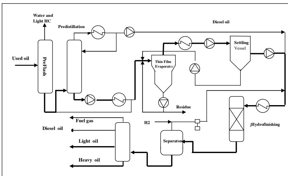
Figure 9 KTI simplified process flow diagram
