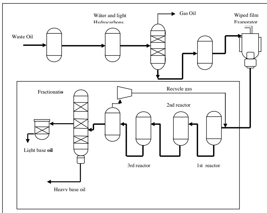
Figure 10 CEP simplified process flow diagram source: CEP
