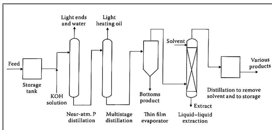
Fig (14) - Dollbergen Process - Source 1, 24
