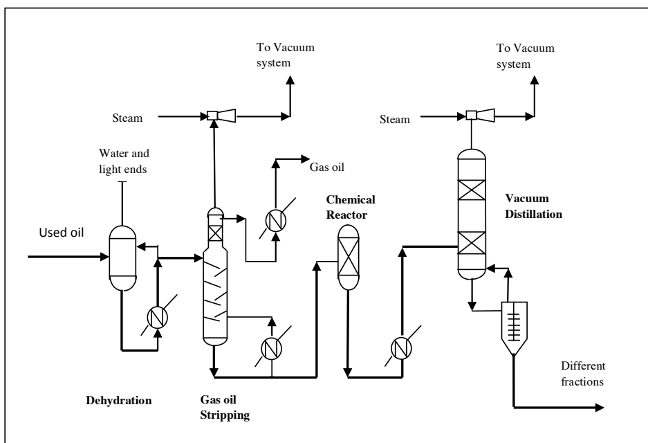
Figure 13 STP simplified process flow diagram Source STP
