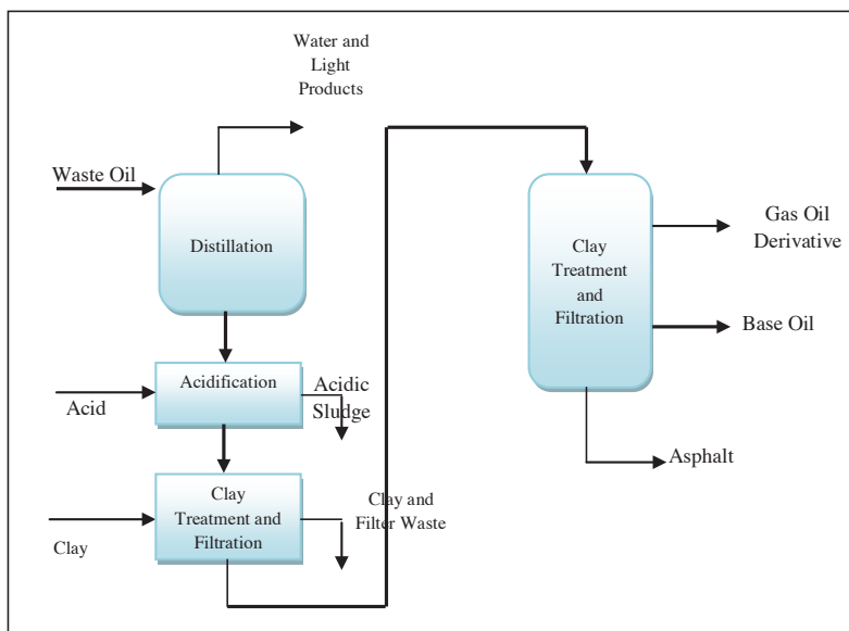
Figure 21 Acid/Clay re-refining process
