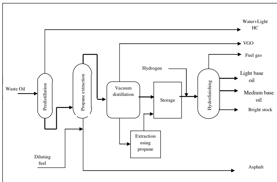
Figure 17 Snamprogetti simplified process flow diagram
