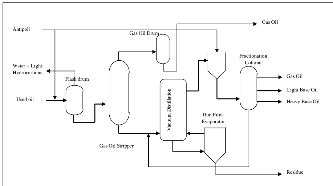
Figure 24 SOTULUB simplified process flow diagram
