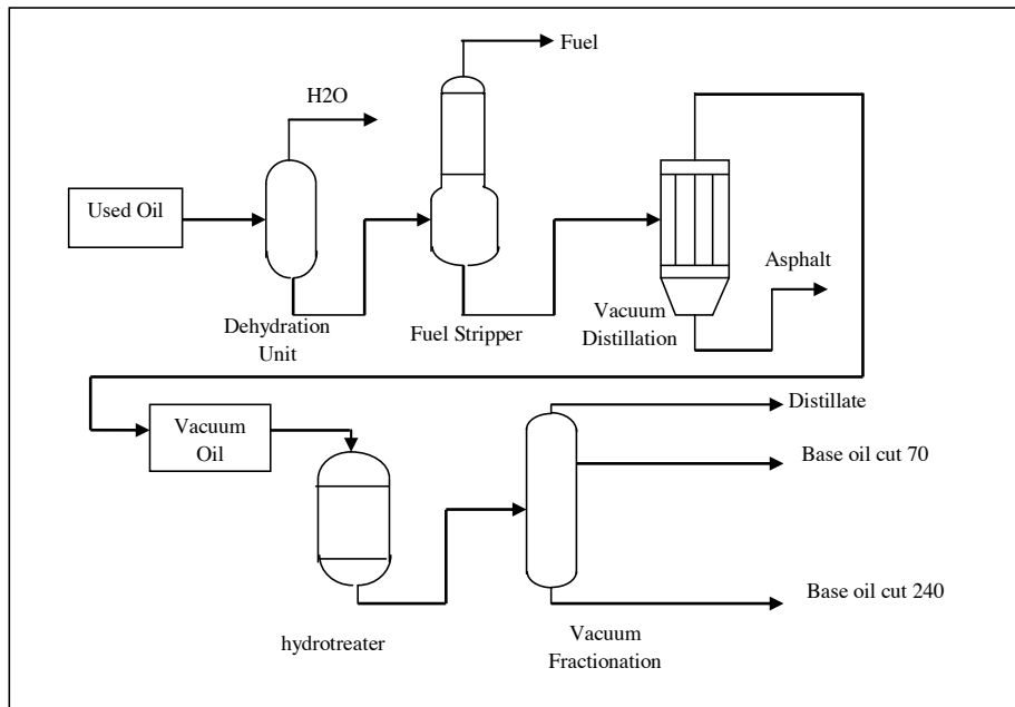
Figure 8 Safety Kleen simplified process flow diagram
