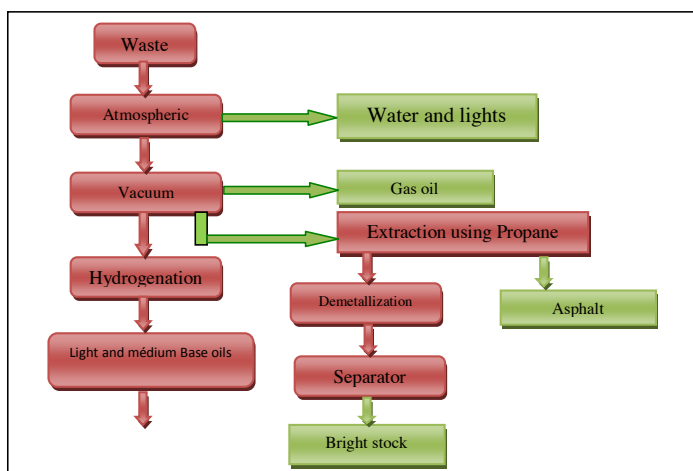
Figure 16 IFP simplified block flow diagram
