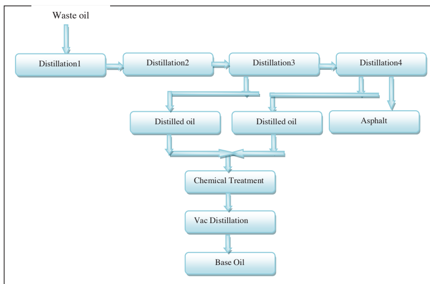
Figure 18 Schematic of the VAXON re-refining process Source UNEP (2012)
