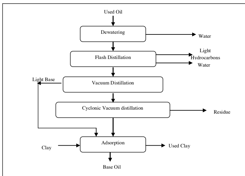
Figure 23 RTI simplified block flow diagram Source Giovana et al (2003)
