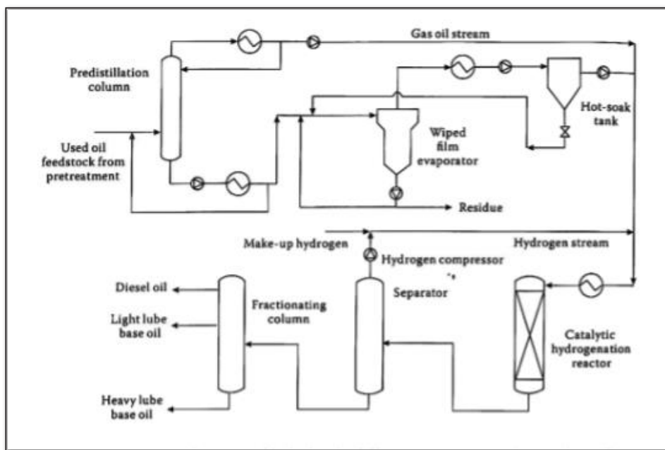
Fig (11) - The KTI Process - Source 1
