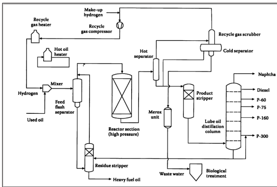
Fig (12) - The Hylube Process - Source 1
