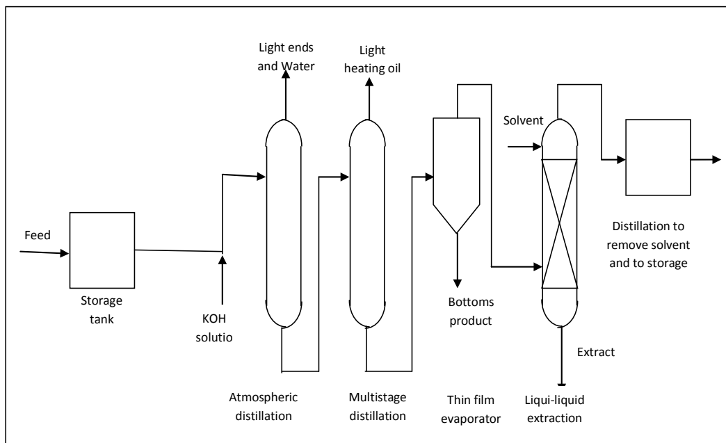
Figure 25 MRD simplified process flow diagram
