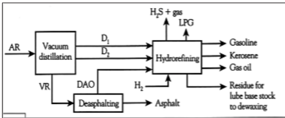
Fig (2) Alternative Virgin Base Oil Processing Source: 2
