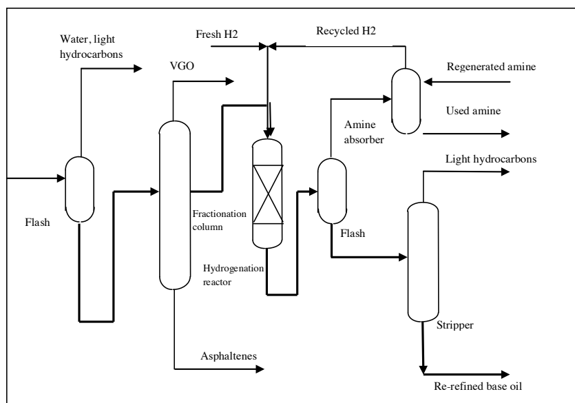
Figure 12 Revivoil simplified process flow diagram Source: Petder (2012)
