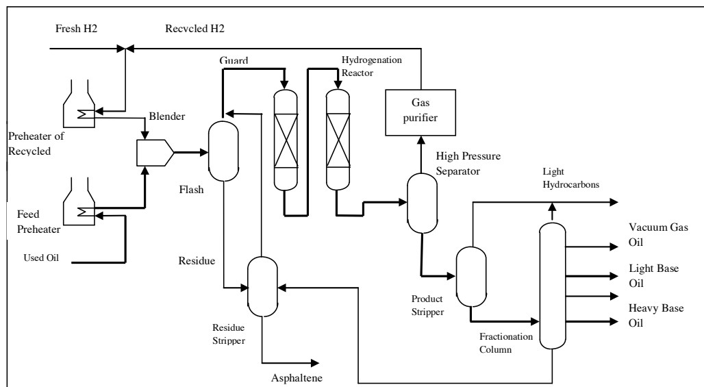
Figure 11 UOP Hylube simplified process flow diagram
