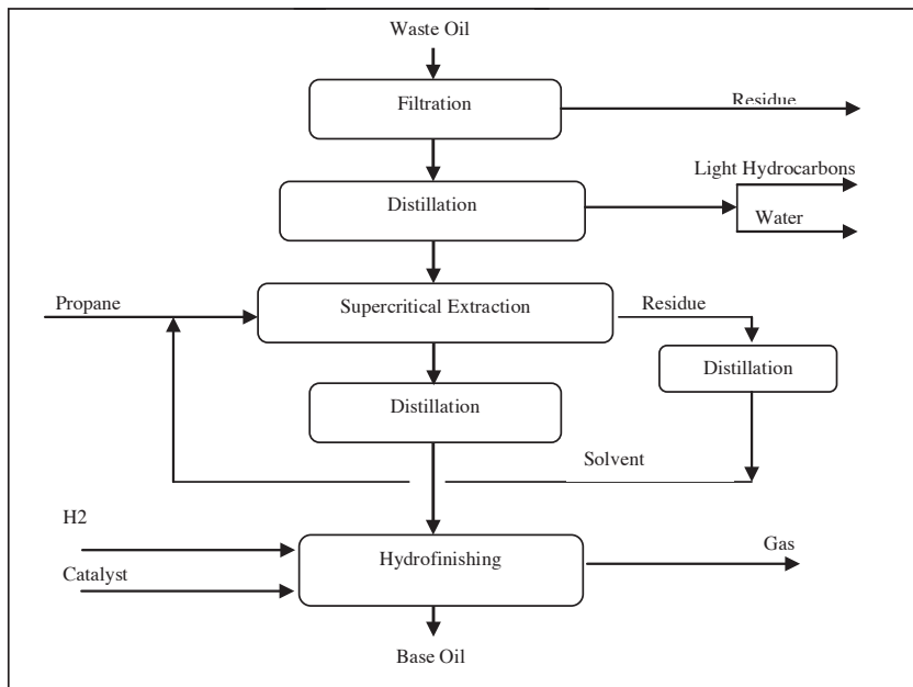
Figure 20 ROSE/Kellog simplified block flow diagram; Source Giovanna et al (2003)
