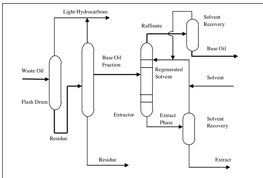
Figure 13 STP simplified process flow diagram Source STP
