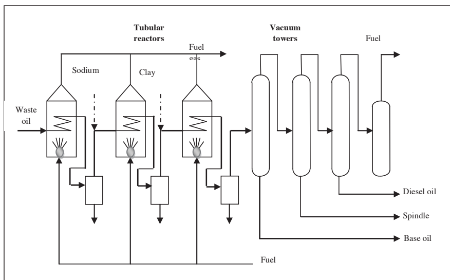
Figure 22 ENTRA simplified process flow diagram
