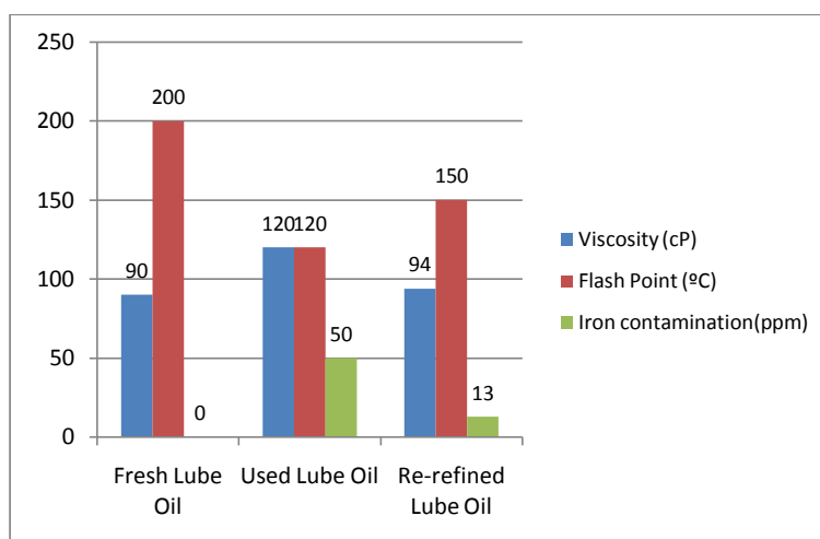
Figure 7 Comparison of Viscosity, Flash Point and Iron content before and after re-refining. Source: own elaboration with data from (Abro et Al, 2013)
