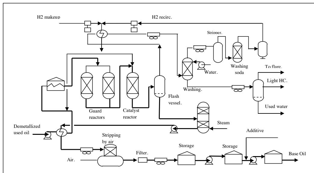
Figure 15 PROP process process flow sheet Source: Audibert as cited in UNEP (2012)
