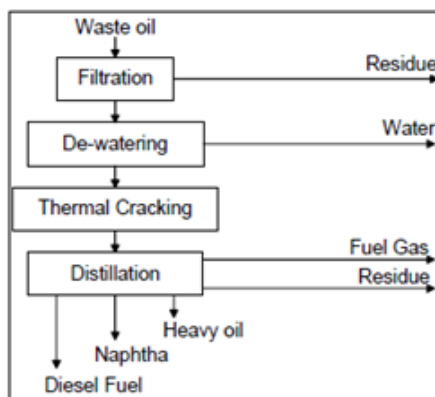
Fig (18) – SOC process – Source 107
