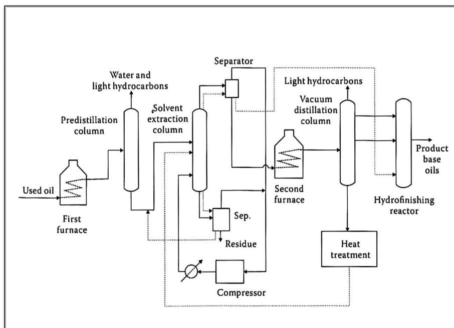
Fig (10) - Snamprogetti Process - Source 1, 3
