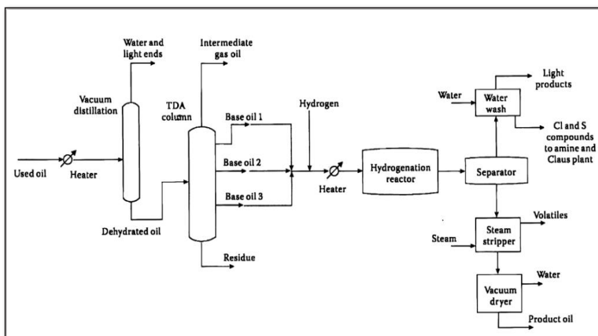
Fig (9) - Simplified Revivoil Process - Source 1
