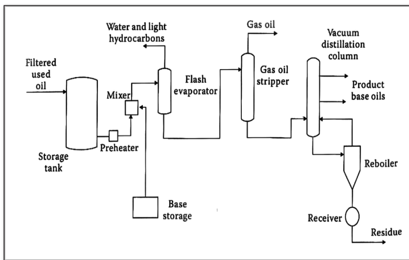
Fig (4) – Sotulub Process – Source 1
