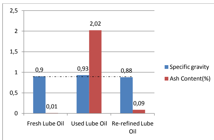
Figure 6 Comparison of Specific Gravity and Ash content before and after re-refining
