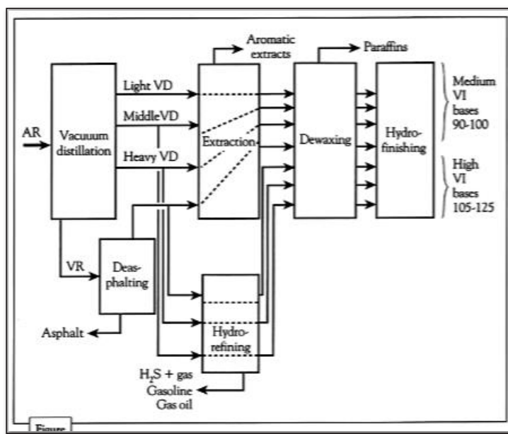
Fig (1) Virgin Lube Processing - Source: 2
