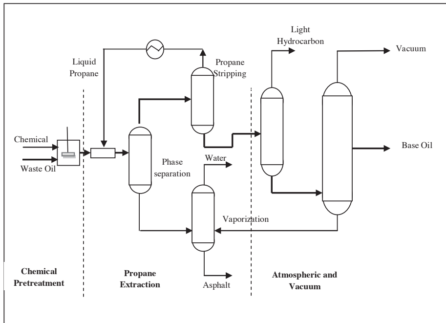
Figure 19 Interline simplified process flow diagram
