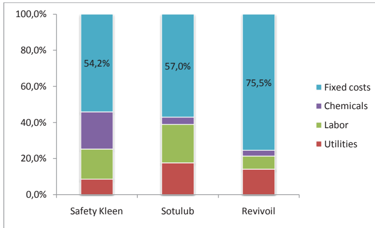
Figure 30 Operating costs for different re-refining technologies Source: Own elaboration with data from (Audibert, 2006)
