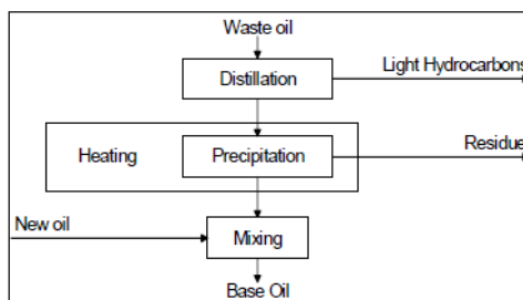
Fig (17) – Zimmark Process – Source 107
